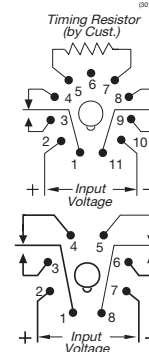
PIN CONFIGURATION Polarity Shown is for D.C. Models
