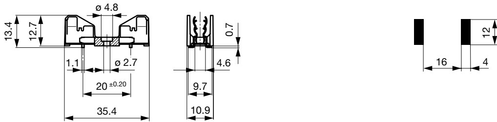
Solder pads
