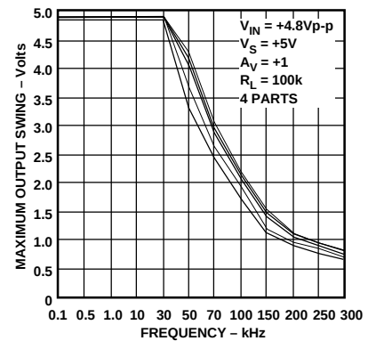
Figure 37. Maximum Output Swing vs. Frequency, V_S = +5V
