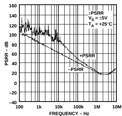
Figure 49. PSRR vs. Frequency, V_S = \pm 5V
