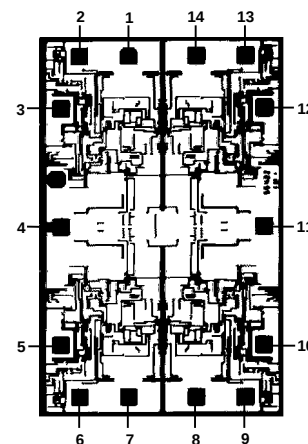
OP491 Die Size 0.070 \times 0.110\text{ Inch} , 7,700 Sq. Mils. Substrate (Die Back- side) Is Connected to V_+ . Transistor Count, 290.
