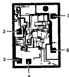
OP191 Die Size 0.047 \times 0.066\text{ Inch} , 3,102 Sq. Mils. Substrate (Die Back- side) Is Connected to V_+ . Transistor Count, 74.
