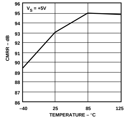
Figure 31. CMRR vs. Temperature, V_S = +5V
