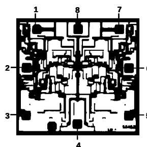
OP291 Die Size 0.070 \times 0.070\text{ Inch} , 4,900 Sq. Mils. Substrate (Die Back- side) Is Connected to V_+ . Transistor Count, 146
