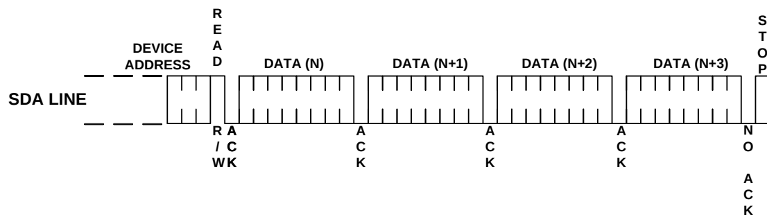
Figure 8: Sequential Read
