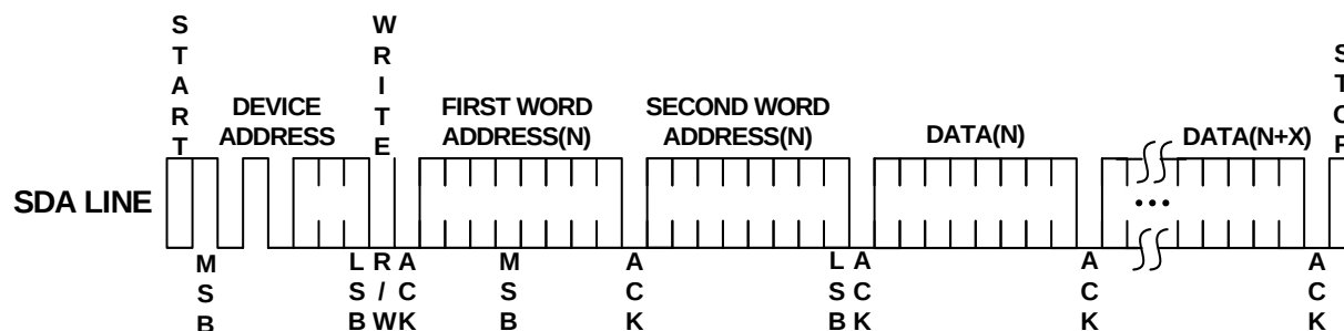
Figure 6: Page Write
