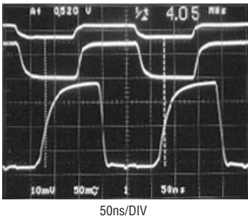
Figure 10. Adaptive Trigger Responding to a 4MHz, 5mV Input. Input Amplitude Variations from 2mV to 175mV Are Accommodated
