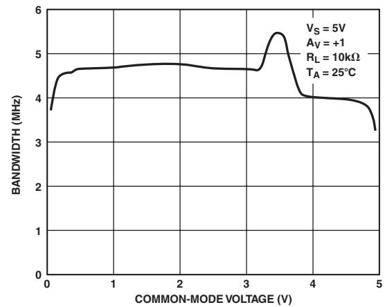
TPC 23. Frequency vs. Common-Mode Voltage ( V_S = 5.0\text{ V} )
