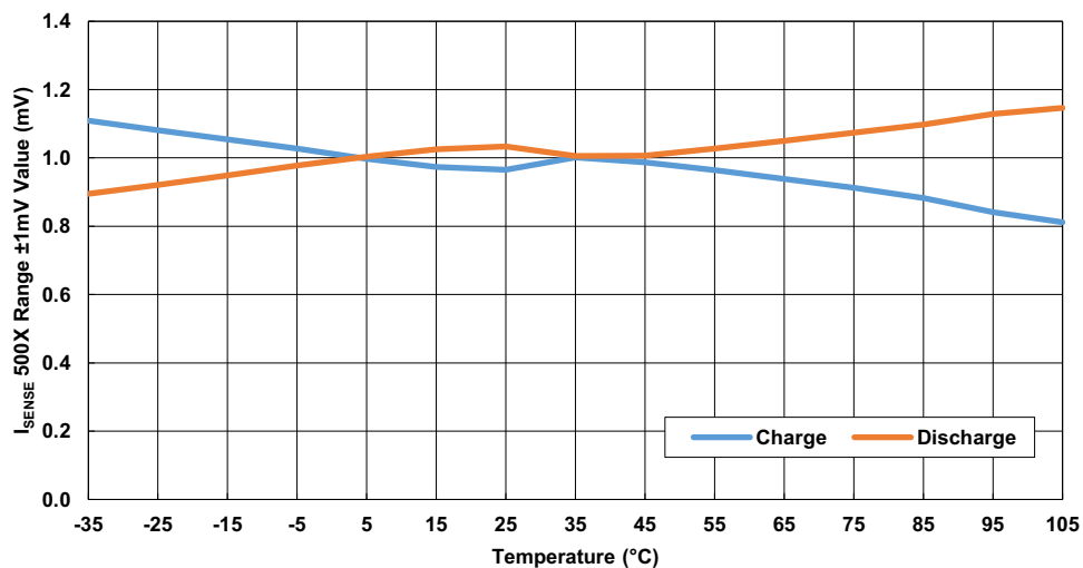
Figure 26. I_{\text{SENSE}} Voltage 500x Gain (1mV) vs Temperature
