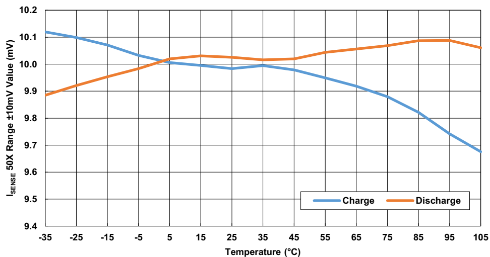
Figure 27. I_{\text{SENSE}} Voltage 50x Gain (10mV) vs Temperature
