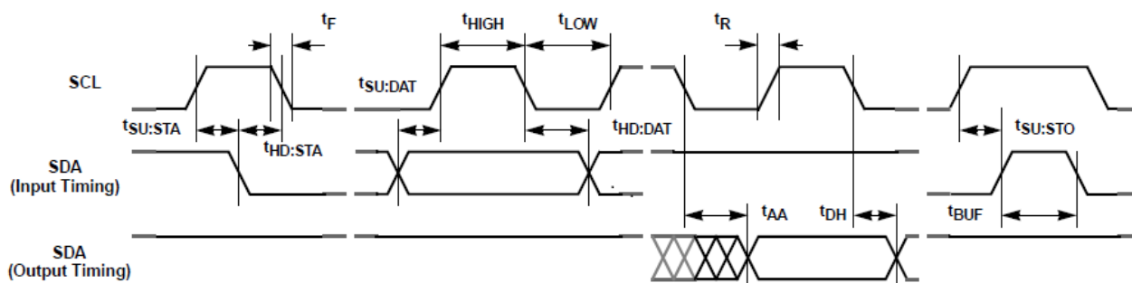
Figure 80. I2C Timing
