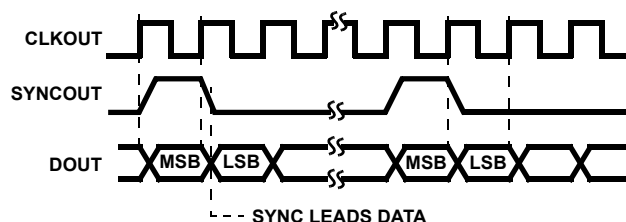
FIGURE 11. SERIAL OUTPUT TIMING
