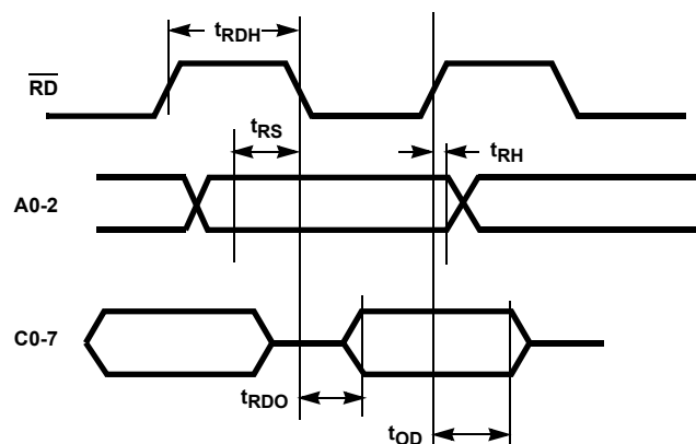
FIGURE 18. TIMING RELATIVE TO READ
