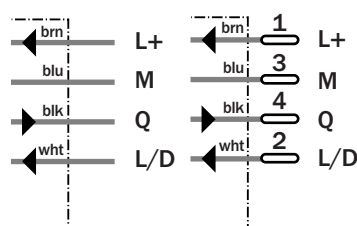
4-pin, M12
