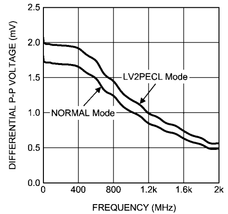
LVPECL VOD vs. Frequency
