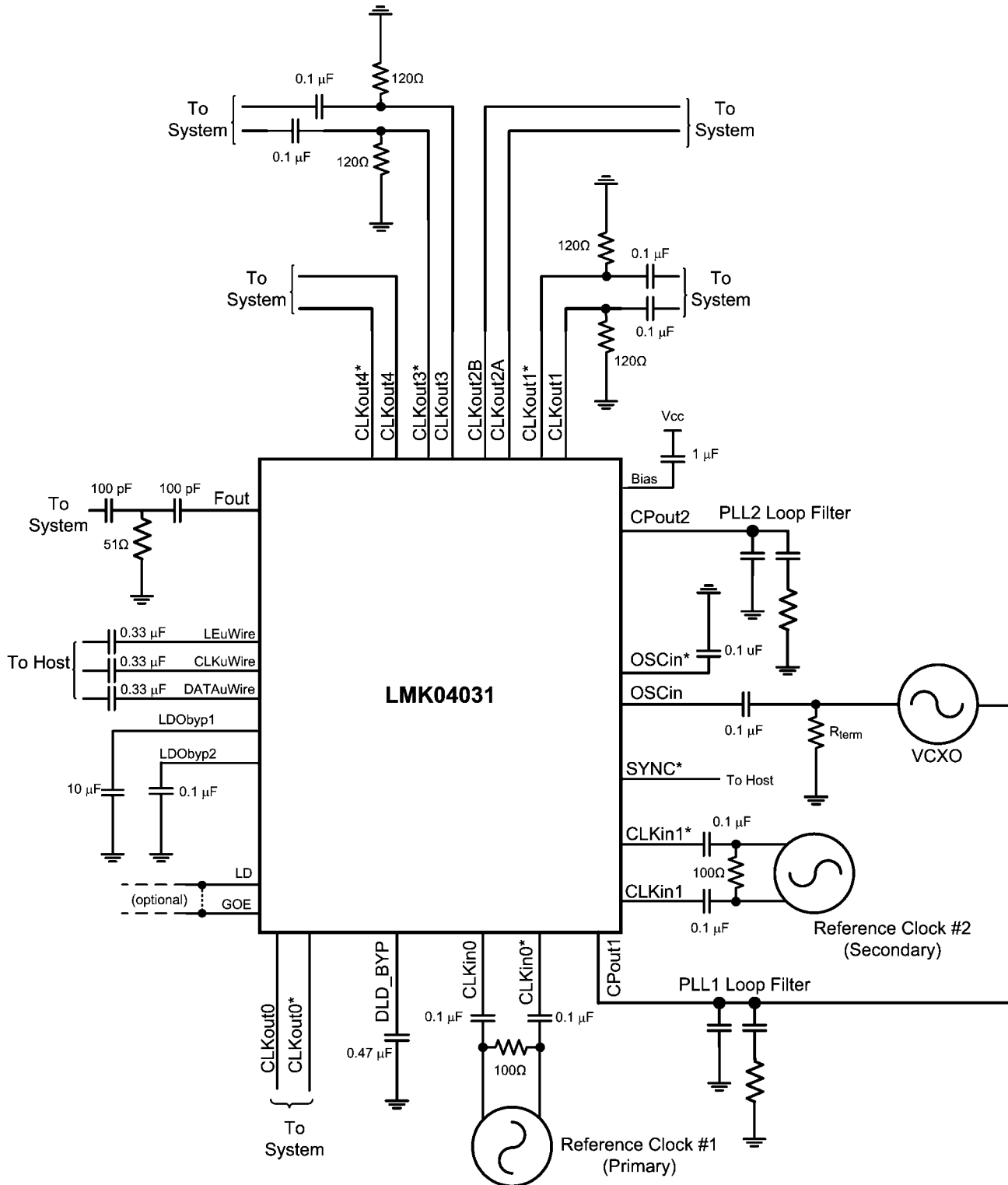
FIGURE 3. Typical Application
