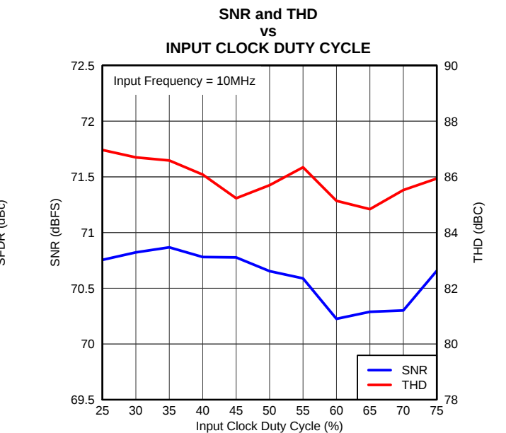
Figure 6-14. Performance Across Input Clock Duty Cycle
