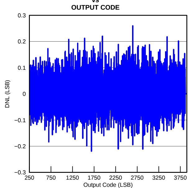
Figure 6-16. DNL Plot
