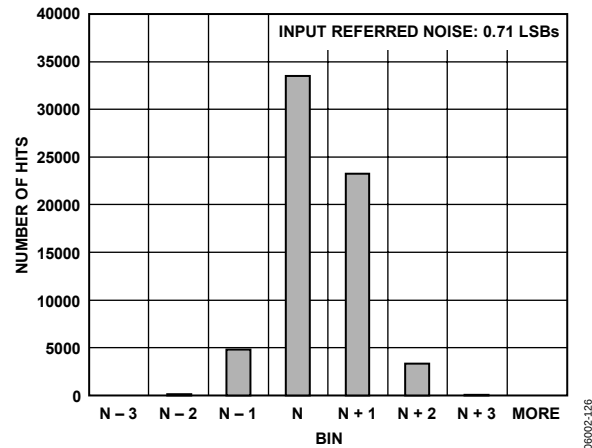
Figure 37. AD9230-250 Grounded Input Histogram; 250 MSPS
