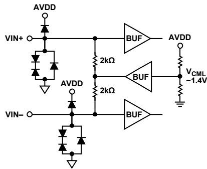
Figure 7. Analog Inputs ( V_{CML} = \sim 1.4\text{ V} )
