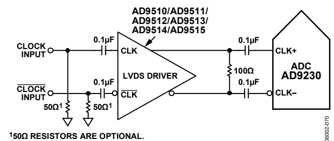
Figure 57. Differential LVDS Sample Clock
