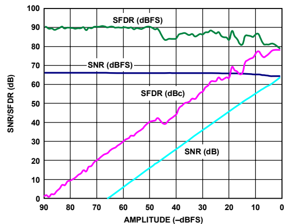
Figure 28. AD9230-210 SNR/SFDR vs. Input Amplitude; 210 MSPS, 170.3 MHz
