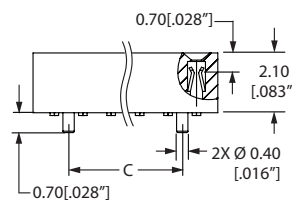
SFM210- SFM315- OPTIONAL GUIDE POSTS REQUIRE (SP) TERMINATION TYPE
