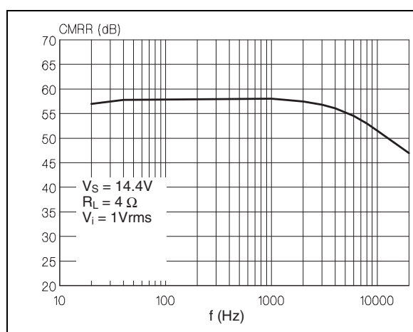
Figure 13. CMRR vs. frequency
