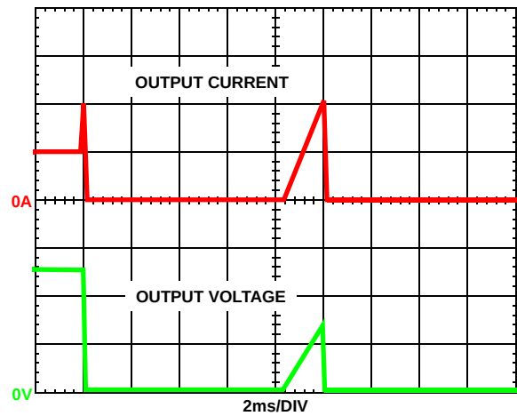
FIGURE 10. OVERCURRENT BEHAVIOR IN HICCUP MODE. F_{SW} = 500kHz
