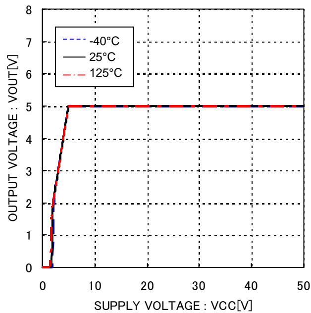
Figure 17. Output voltage vs. Supply voltage IOU=100mA
