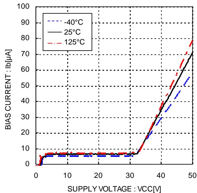
Figure 5. Bias current
