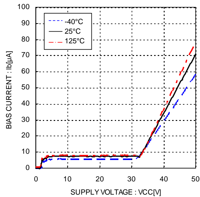
Figure 15. Bias current
