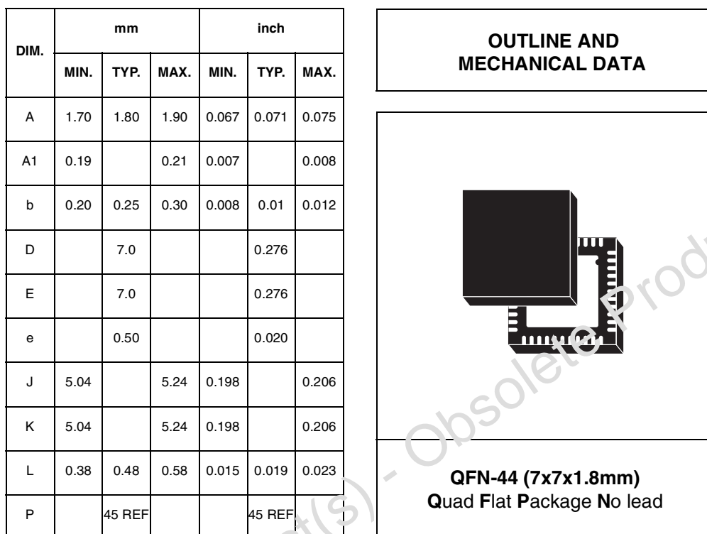
Figure 21. QFN-44 Mechanical Data & Package Dimensions
