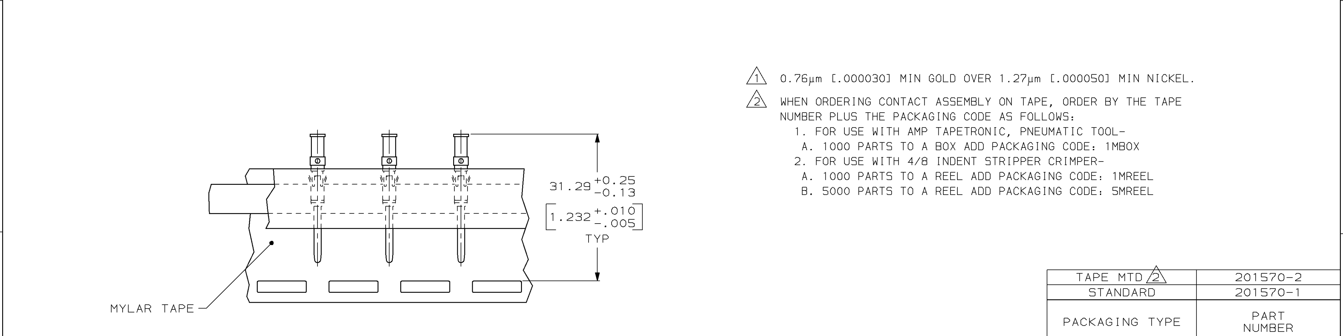
TAPE MTG DETAIL SCALE 2:1
