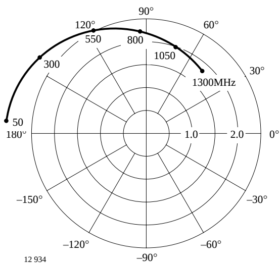
Figure 10. Forward transmission coefficient
