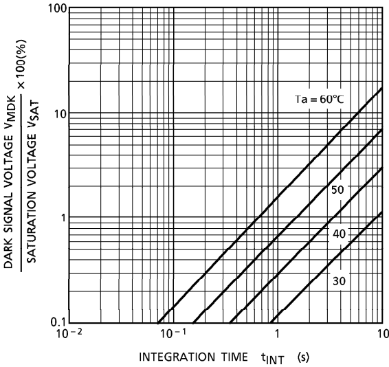
DARK SIGNAL VOLTAGE – INTEGRATION TIME
