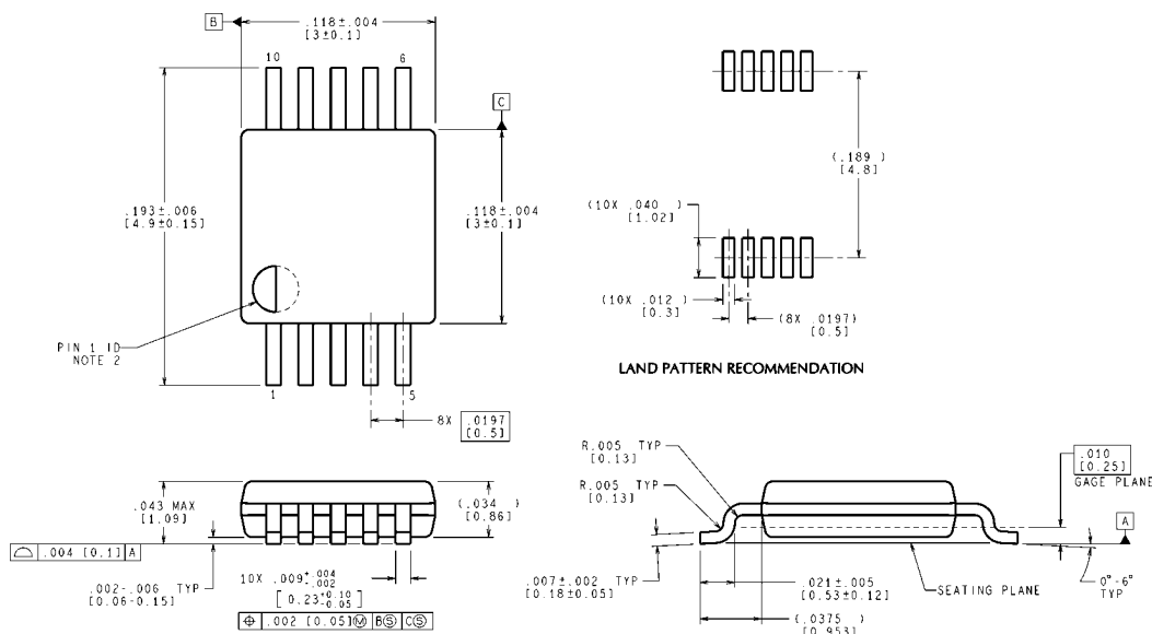
10-Lead MSOP Order Numbers DAC124S085CIMM NS Package Number MUB10A
