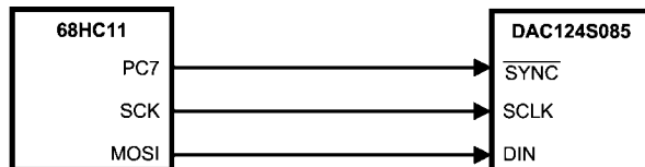
FIGURE 12. 68HC11 Interface
