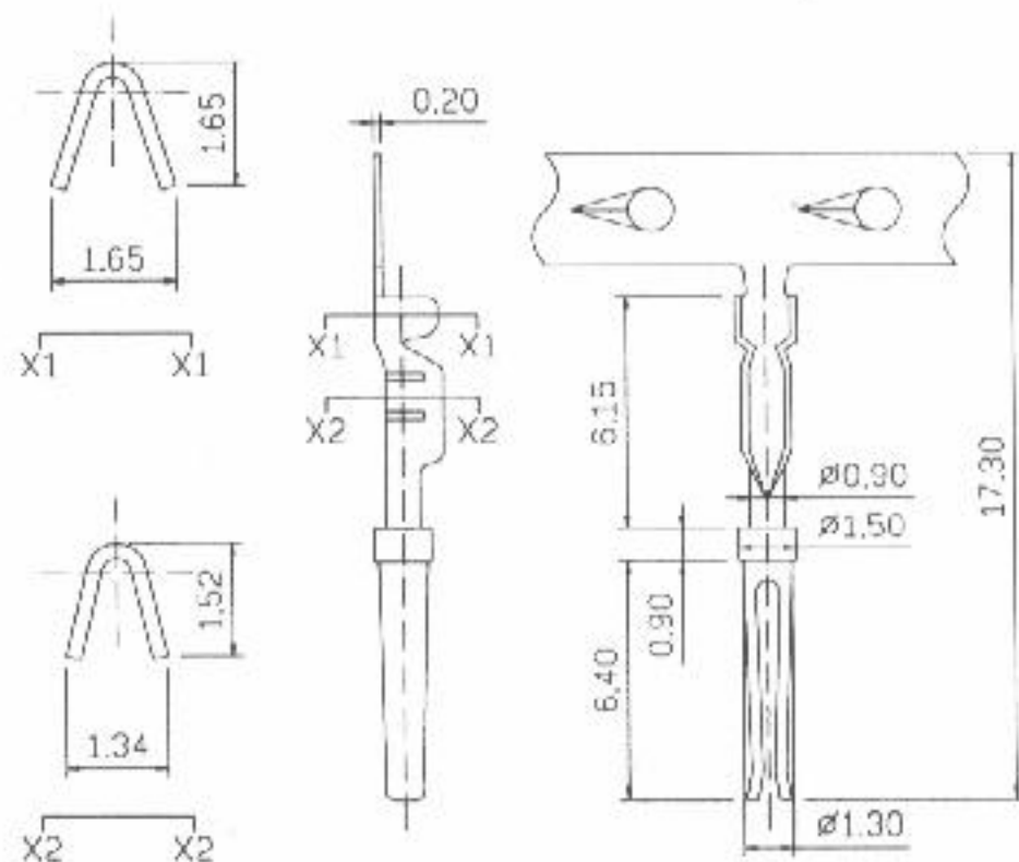
0.76 Crimp Pin Female
