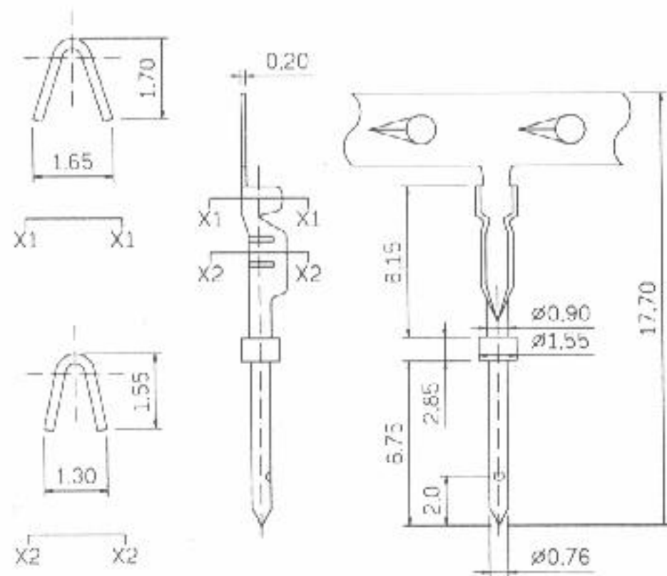
0.76 Crimp Pin Male
