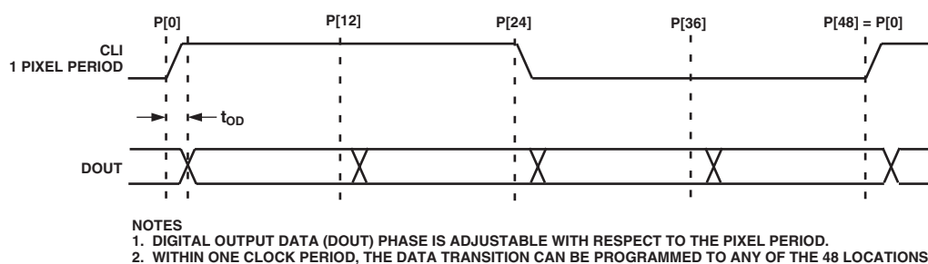
Figure 7a. Digital Output Phase Adjustment
