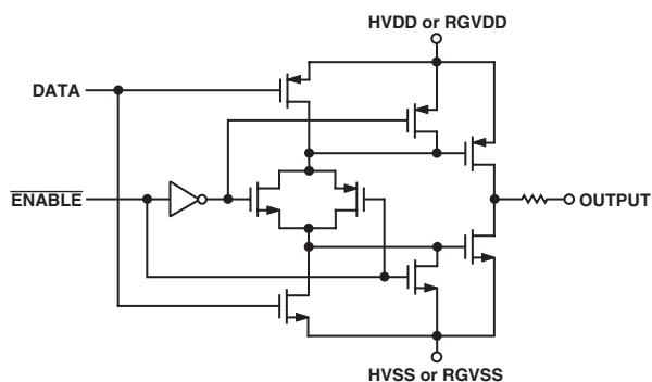
Circuit 5. H1-H4 and RG (Pins 14, 15, 18, 19, 21)
