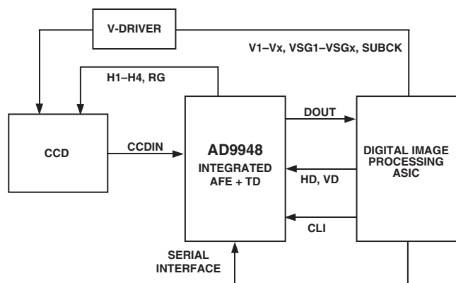
Figure 1. Typical Application
