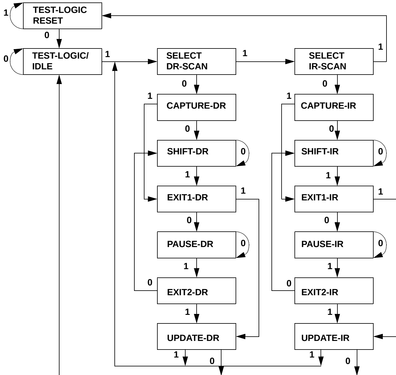
TAP Controller State Diagram [6]
