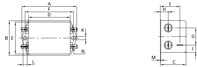
Connection style -06, 16A types
