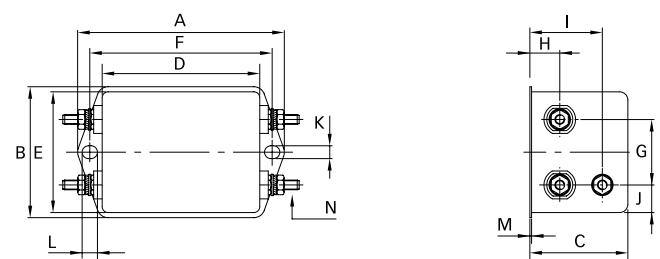
Connection style -08, 16A types
