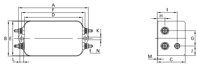
Connection style -08, 20A types
