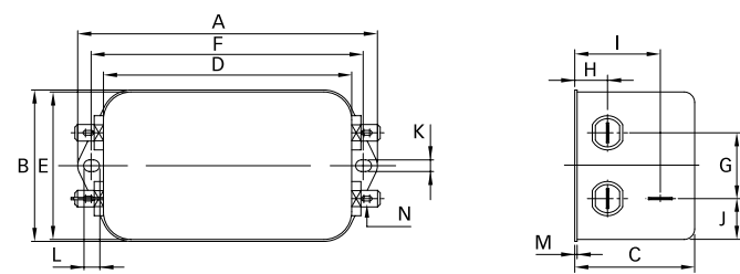
Connection style -06, 20A types
