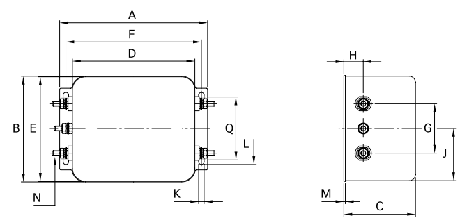
Connection style -08, 30A types
