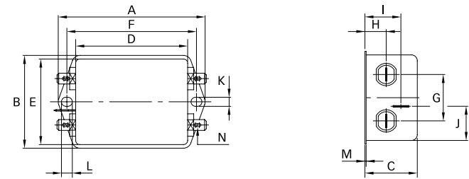
Connection style -06, 1 to 12A types
