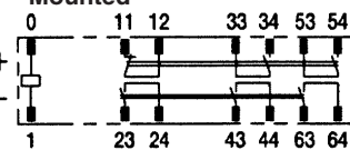
G7SA-5A1B Mounted
