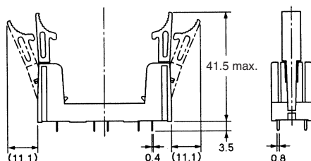
G7SA-3A1B Mounted
