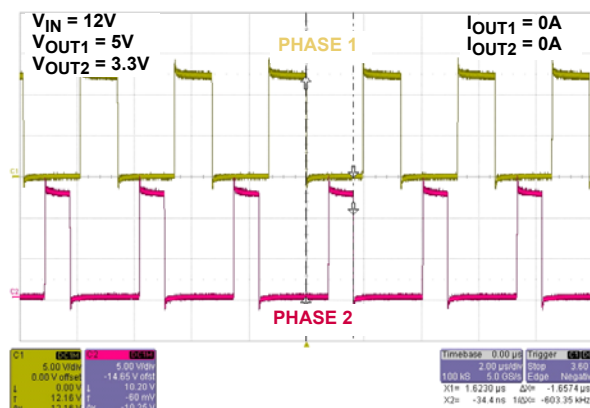
FIGURE 8. PWM INTERLEAVING
