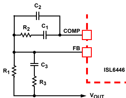
FIGURE 25. COMPENSATION CONFIGURATION FOR ISL6446 CIRCUIT
