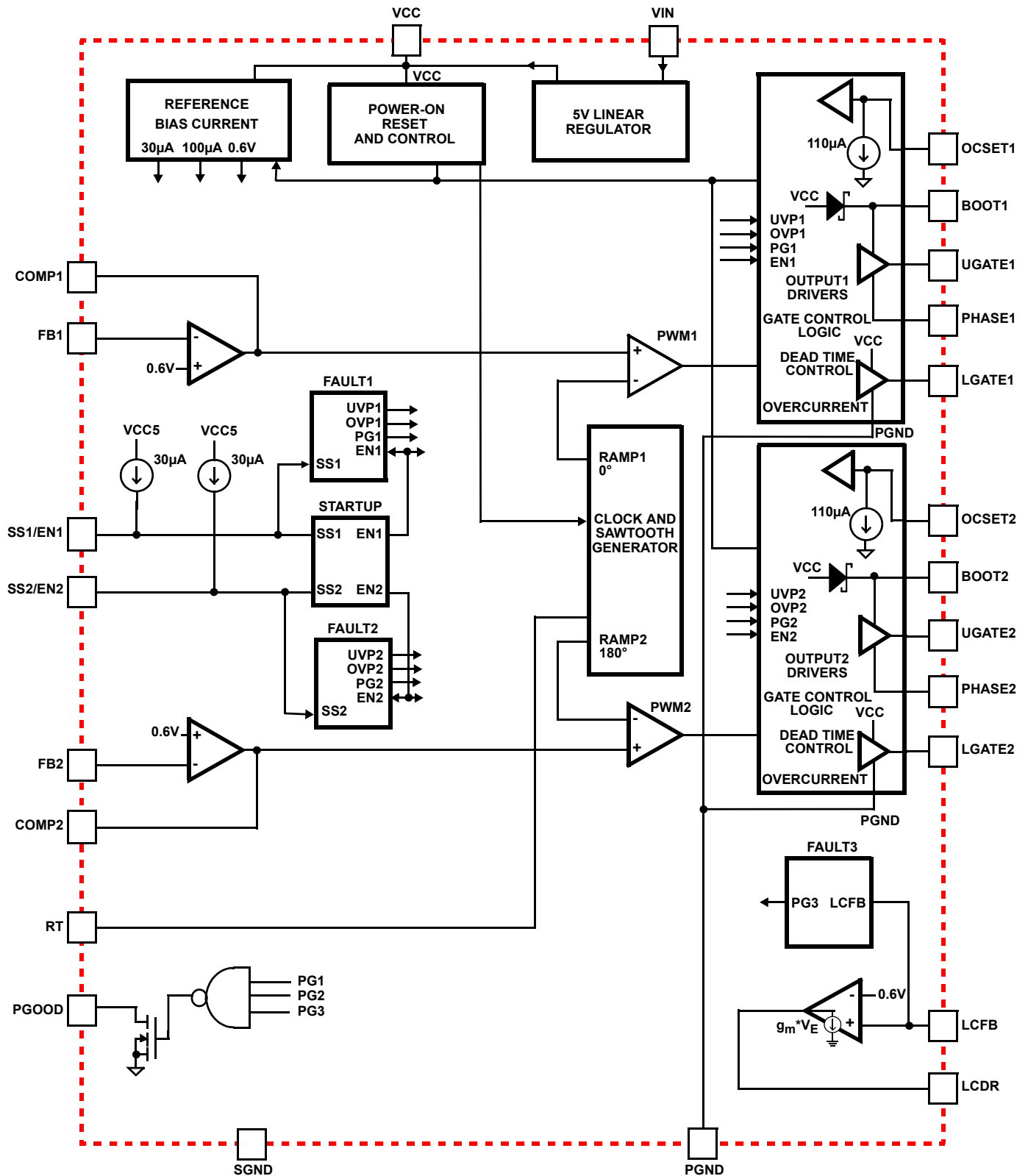
FIGURE 3. BLOCK DIAGRAM
