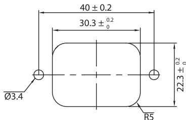
MOUNTING INLET FLANGE AT BACK OF COVER
