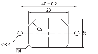
MOUNTING INLET FLANGE IN FRONT OF COVER
