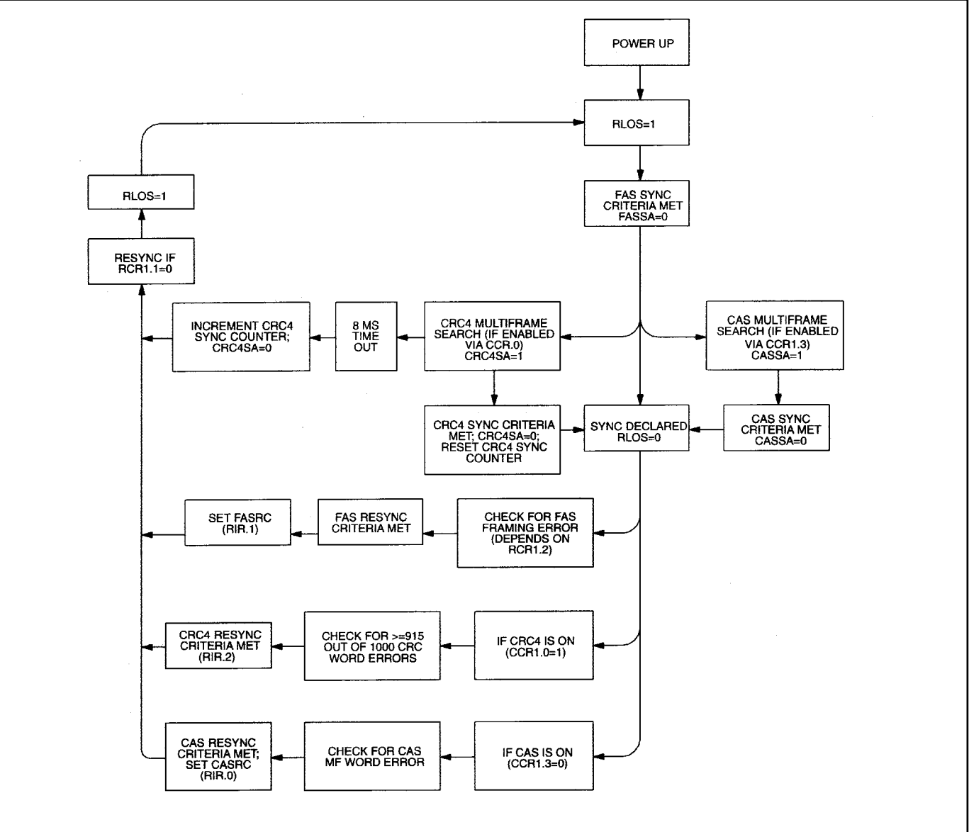
Figure 14-8. Synchronization Flowchart
