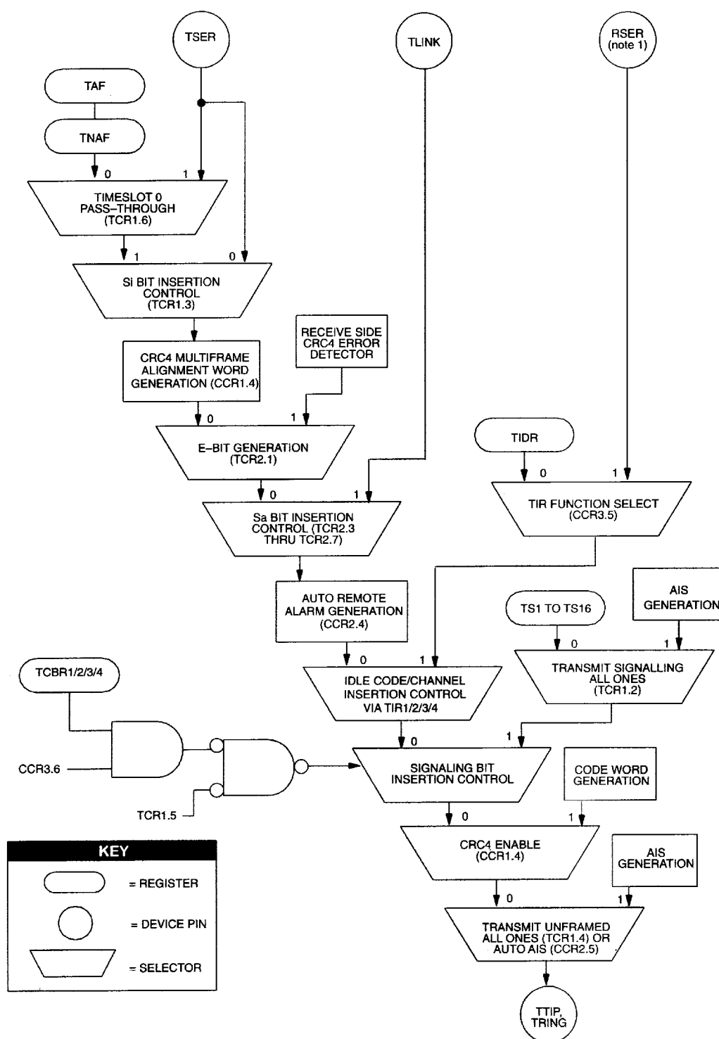
Figure 14-9. Transmit Data Flow
