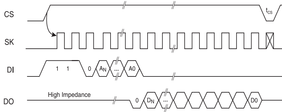
Figure 3. READ Timing
