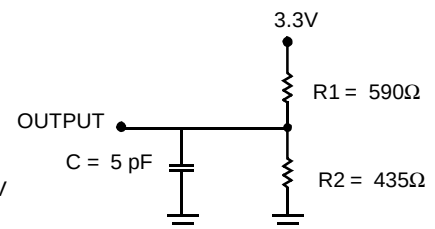
(c) Three-State Delay (Load 2) (Used for t_{LZ} , t_{HZ} , t_{LZWE} & t_{LZWE} including scope and jig)
