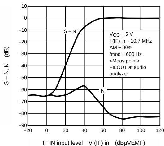
S/N Characteristics (IF input) in the AM Mode
