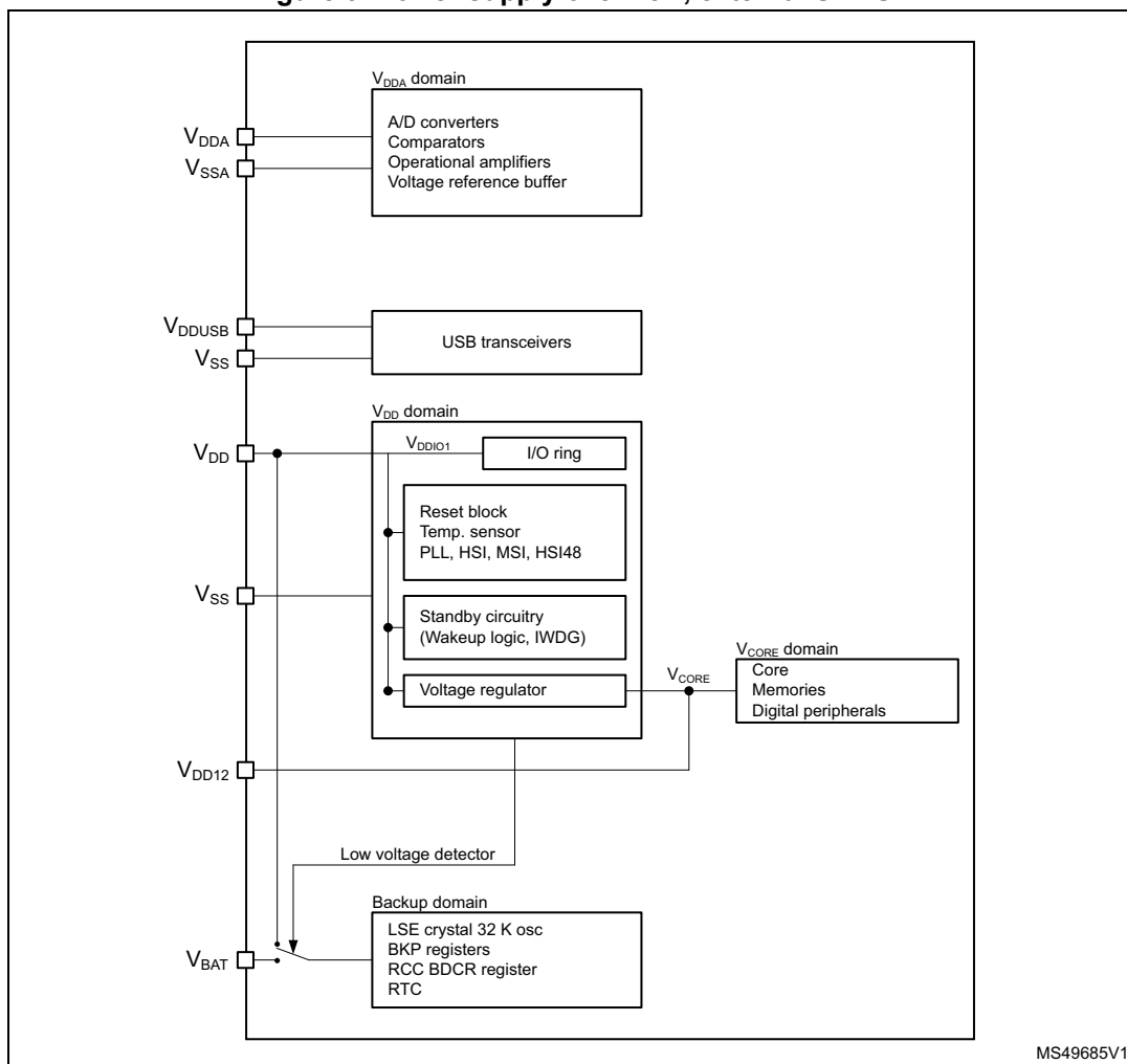
Figure 3. Power supply overview, external SMPS
