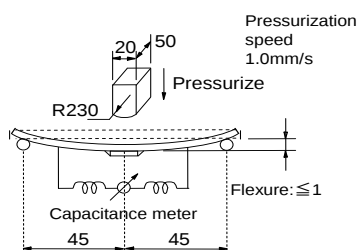
Fig.2 (in mm)
