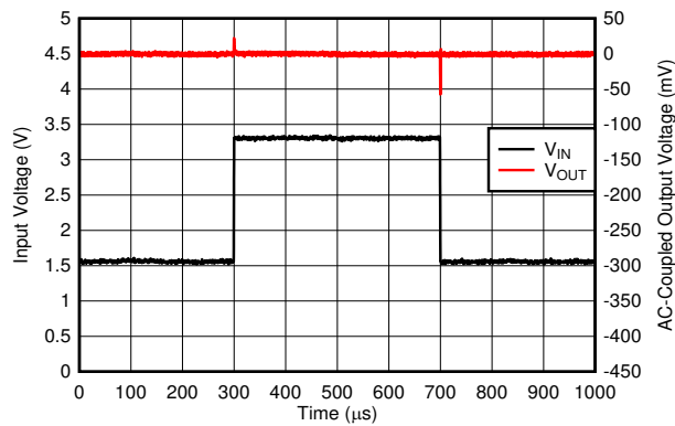
Figure 6-19. V_{IN} Transient
