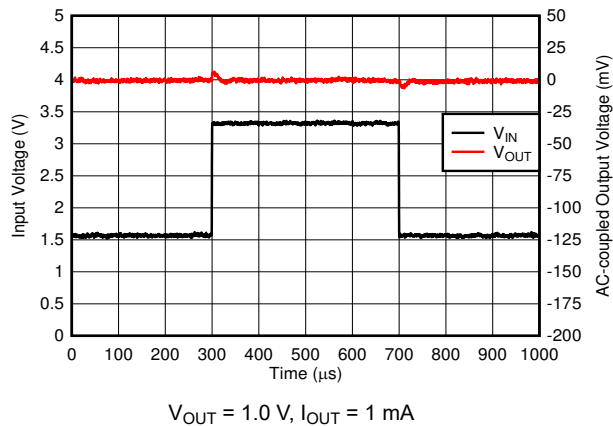
Figure 6-18. V_{IN} Transient
