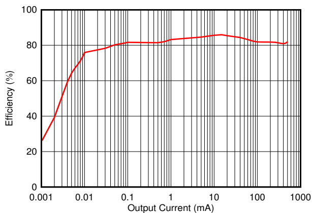
Figure 8-5. TPS7A11 Output Efficiency at 1.2 V_{IN} and 1.0 V_{OUT}
