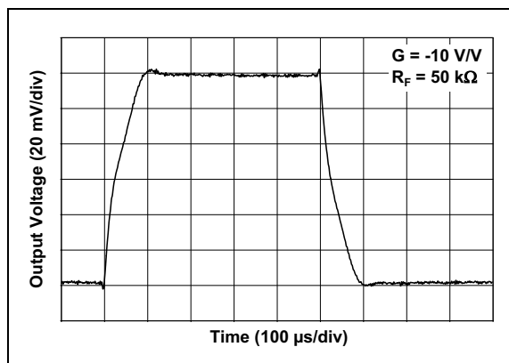
FIGURE 2-30: Small Signal Inverting Pulse Response vs. Time.
