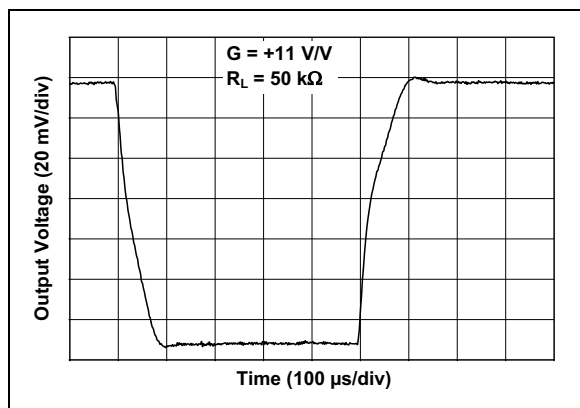
FIGURE 2-27: Small Signal Non-Inverting Pulse Response vs. Time.
