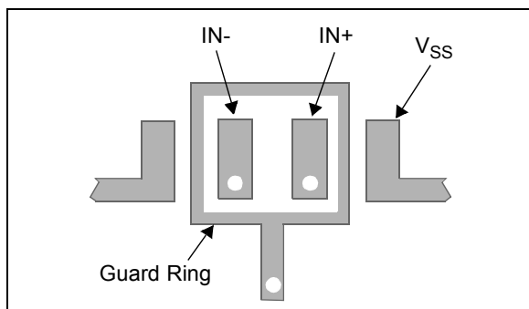
FIGURE 3-6: Example of Guard Ring layout.
