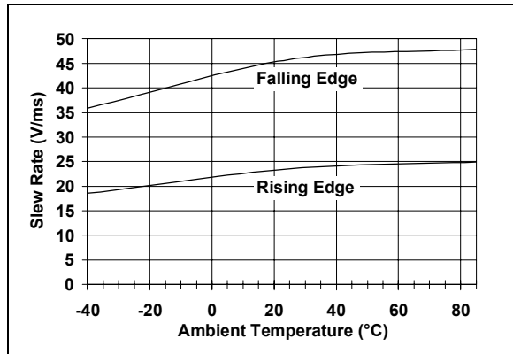
FIGURE 2-25: Slew Rate vs. Ambient Temperature.
