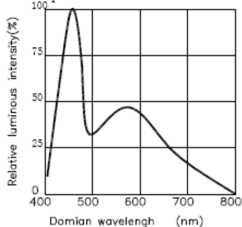
Spectrum Distribution
