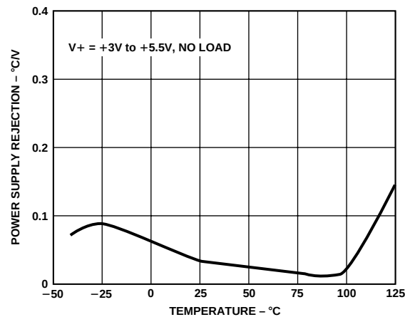
Figure 5. Power Supply Rejection vs. Temperature
