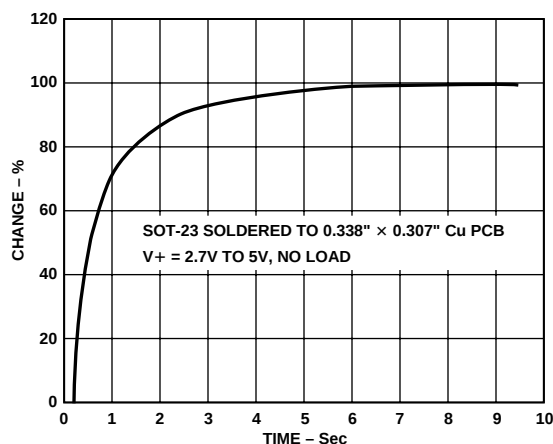
Figure 14. Thermal Response Time in Stirred Oil Bath
