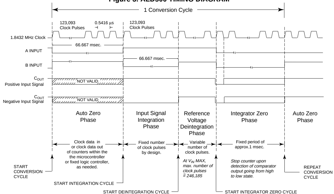
Figure 3. ALD500 TIMING DIAGRAM
