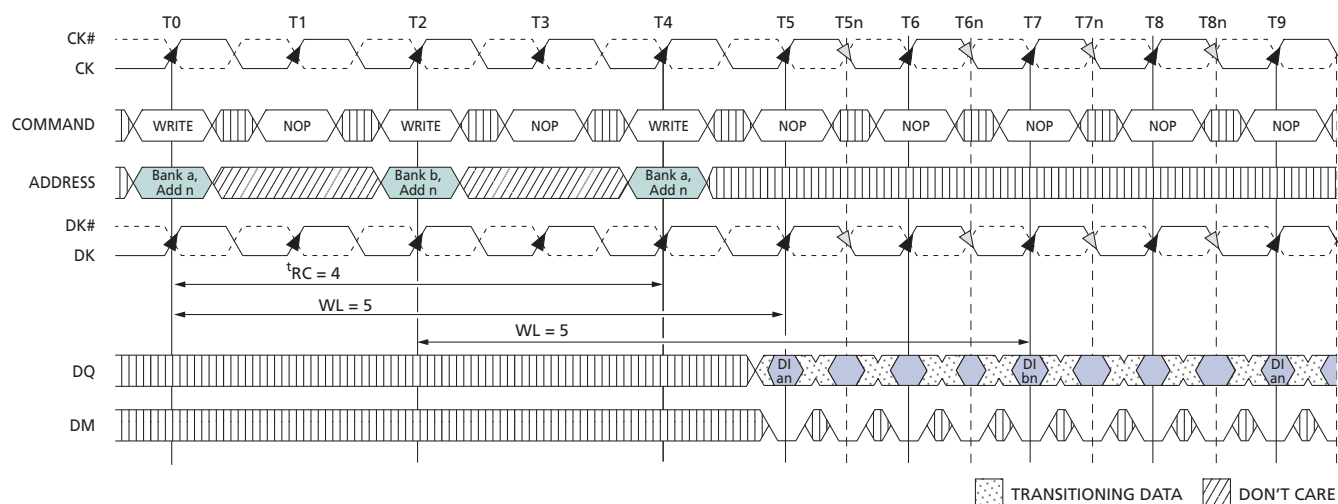
Figure 30: Consecutive WRITE-to-WRITE
