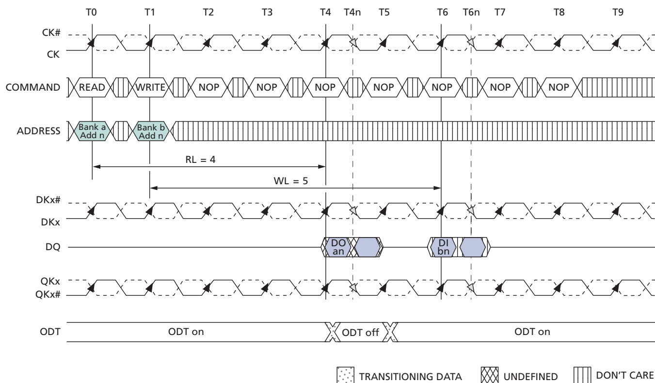
Figure 37: READ-to-WRITE with ODT
