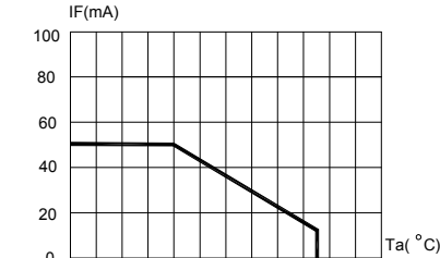
FIG.4a RED MAXIMUM FORWARD DC CURRENT VS AMBIENT TEMPERATURE ( T_{jmax}=105^{\circ}\text{C} )
