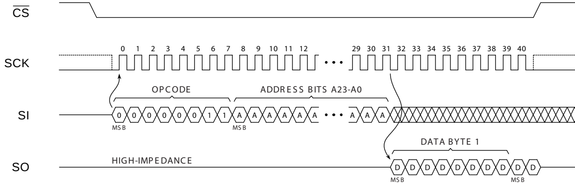
Figure 6-3. Read Array - 03h Opcode
