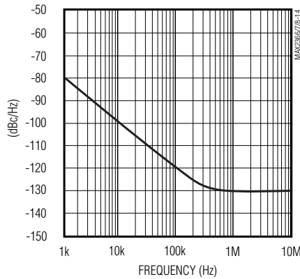
PHASE NOISE HIGH-BAND OSCILLATOR vs. FREQUENCY OFFSET (165MHz)
