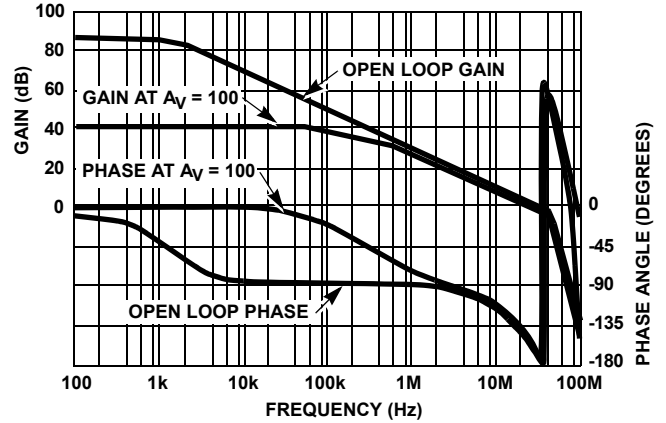
FIGURE 15. FREQUENCY RESPONSE
