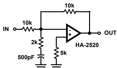
FIGURE 6. INVERTING UNITY GAIN CIRCUIT
