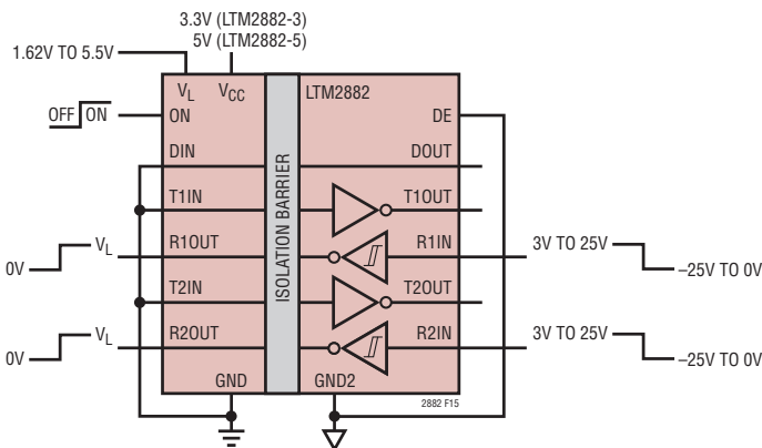
Figure 15. Isolated Dual Inverting Level Translator
