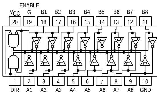
SN54/74LS640 SN54/74LS642
