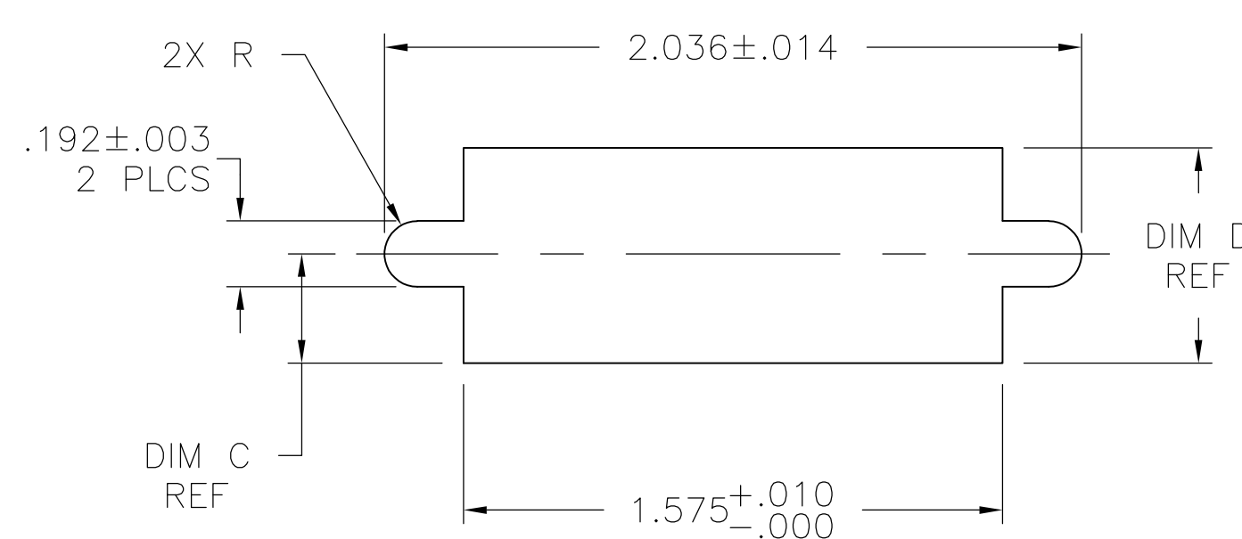
SUGGESTED PANEL CUTOUT FOR METRIC HARDWARE 7 SCALE 4:1
