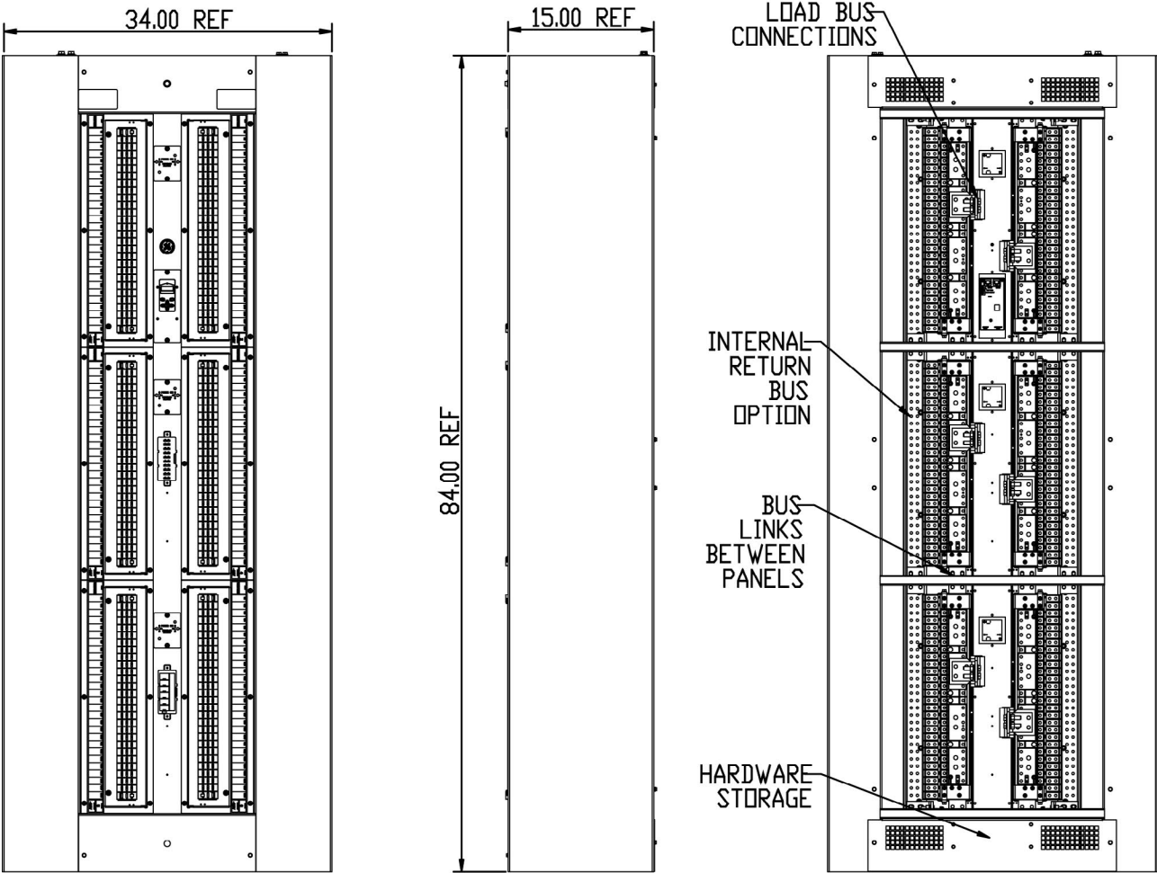
OUTLINE DRAWING OF GROUP 8 (34" WIDE) 7FT CABINET
