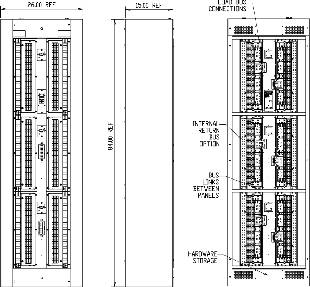
OUTLINE DRAWING OF GROUP 7 (26" WIDE) 7FT CABINET
