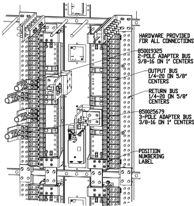
Distribution Panel Connections
