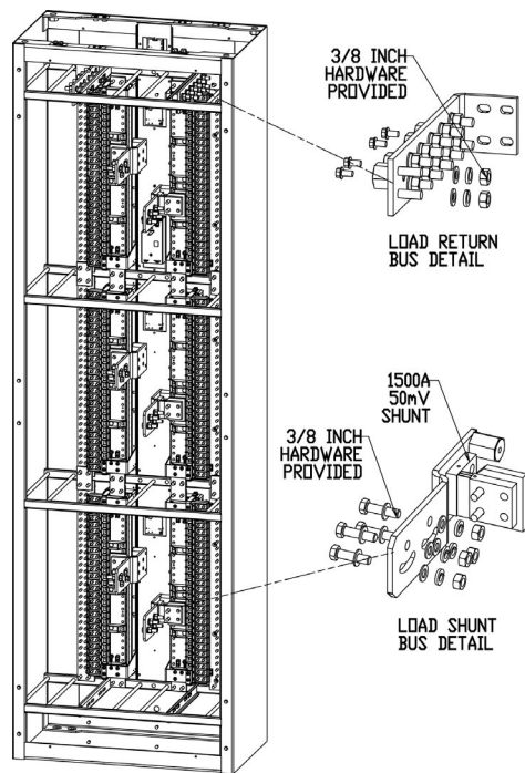
Load Input Connections
