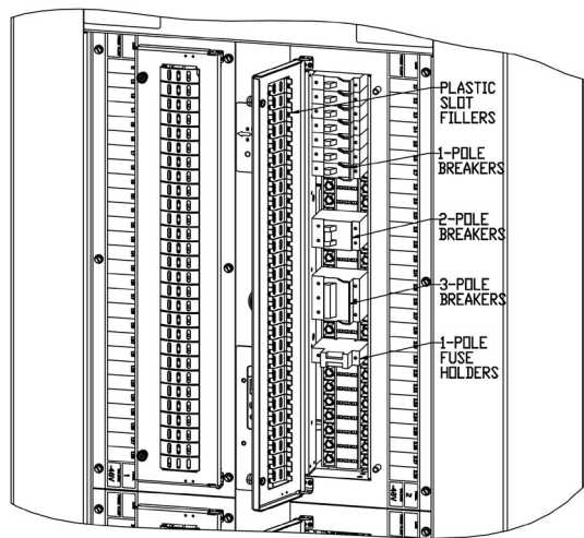
Fuse or Circuit Breaker Installation
