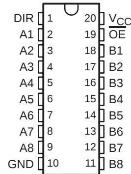
SN54HCT245 . . . J OR W PACKAGE SN74HCT245 . . . DB, DW, N, NS, OR PW PACKAGE (TOP VIEW)
