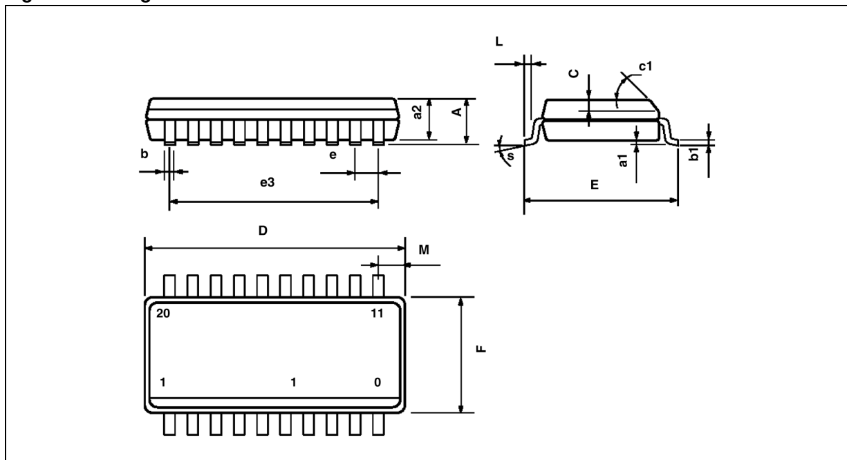
Figure 9. Package Dimensions
