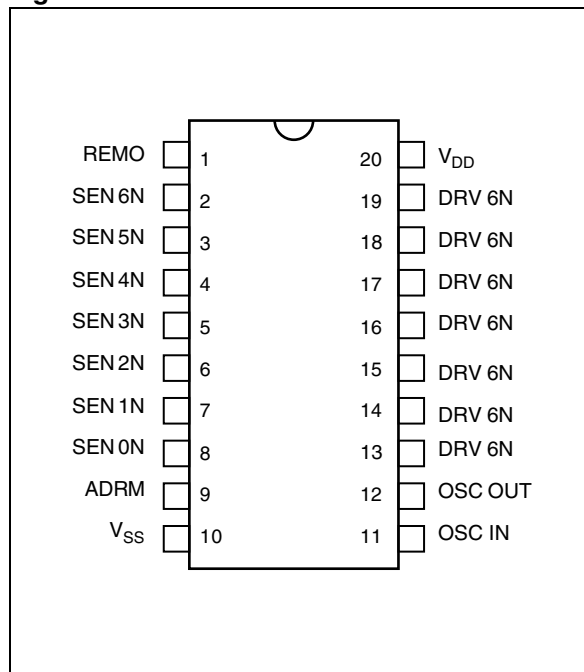
Figure 2. Pin Connection
